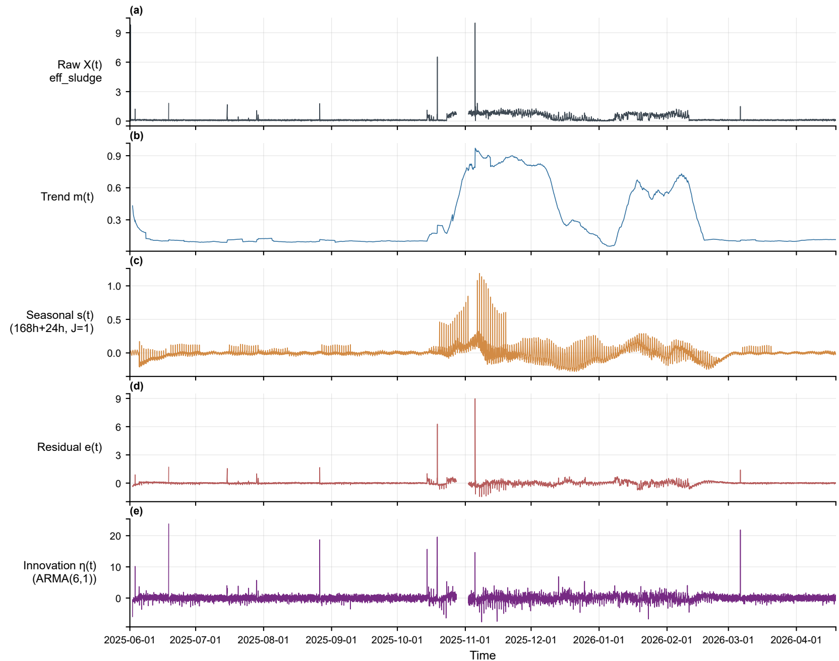
Multi-scale decomposition — eff_sludge (effluent, hour) [2025-06-01~2026-04-19]
